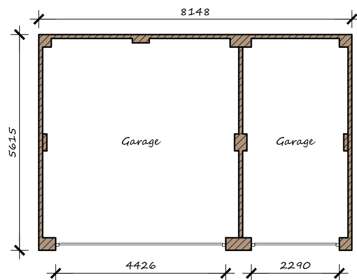
Floor Plan
