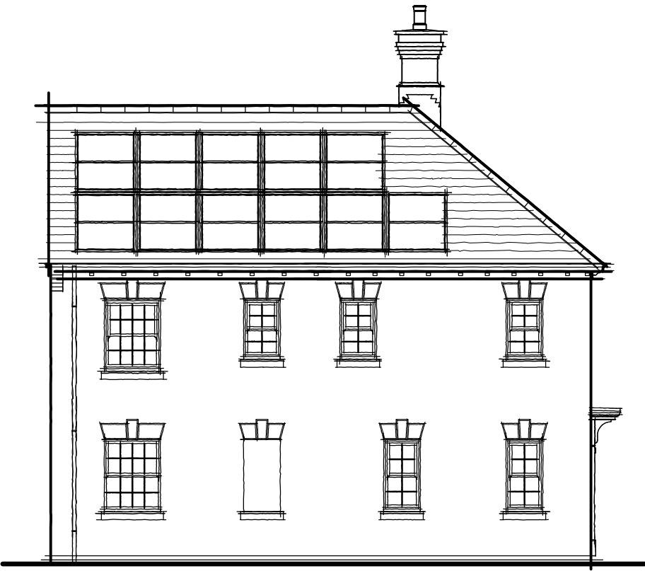
Side Elevation
