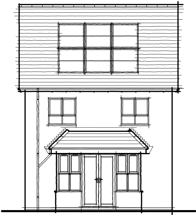
Rear Elevation
