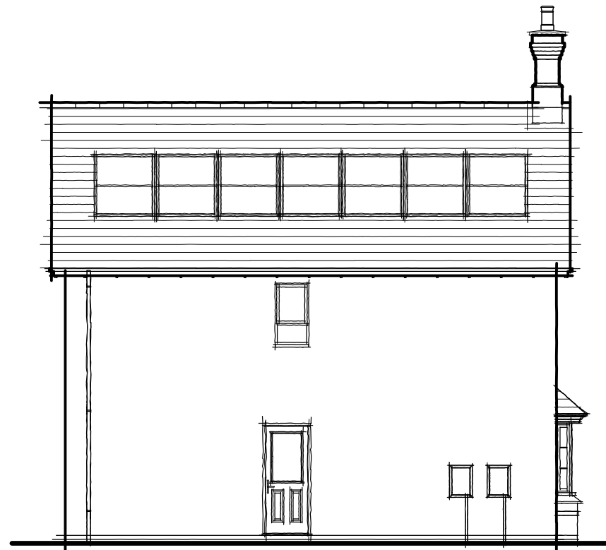
Rear Elevation
