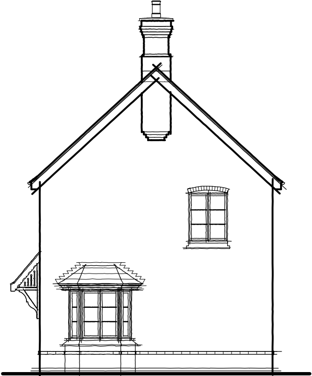
Side Elevation
