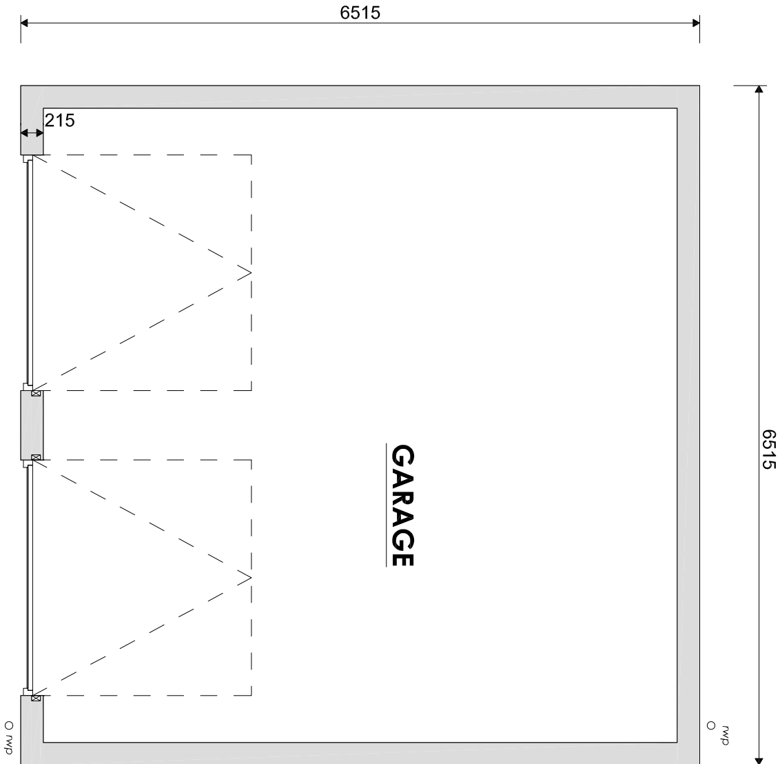
FLOOR PLAN
