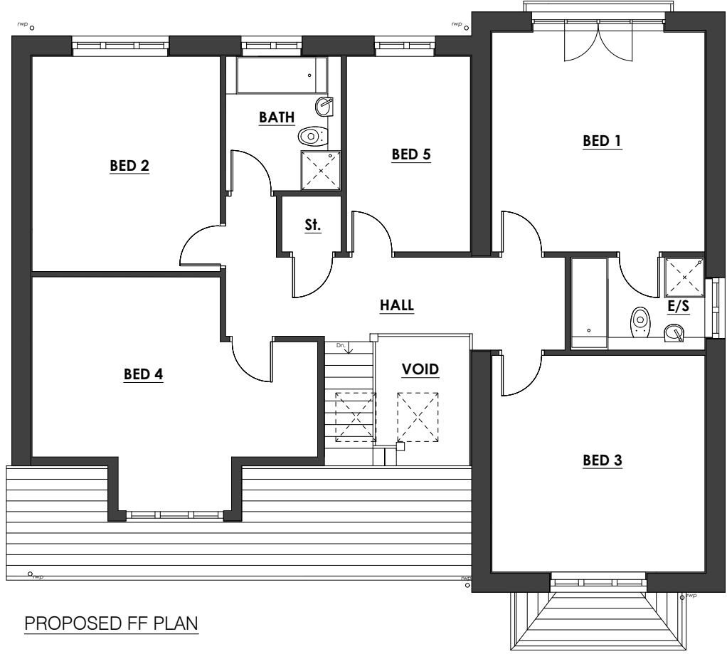
PROPOSED FF PLAN
