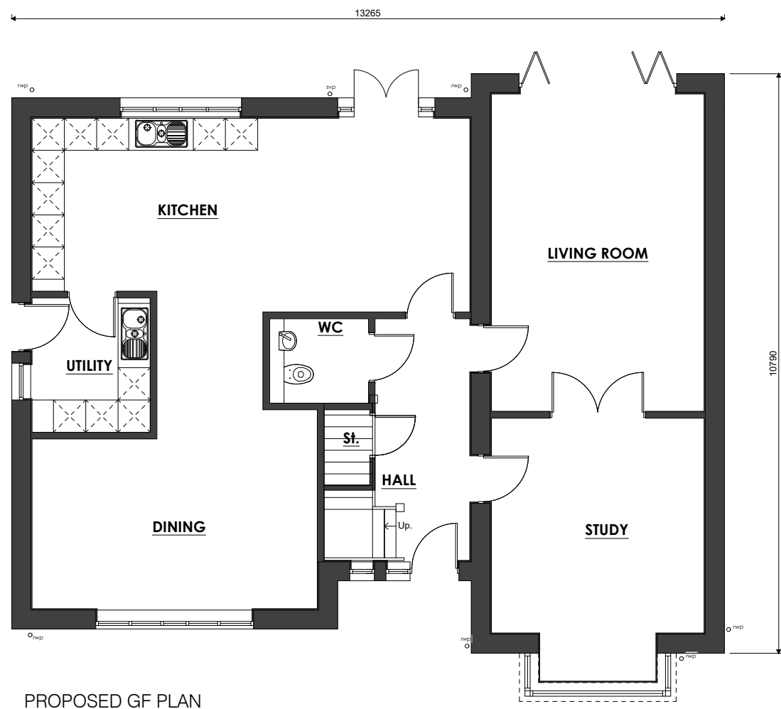
PROPOSED GF PLAN
