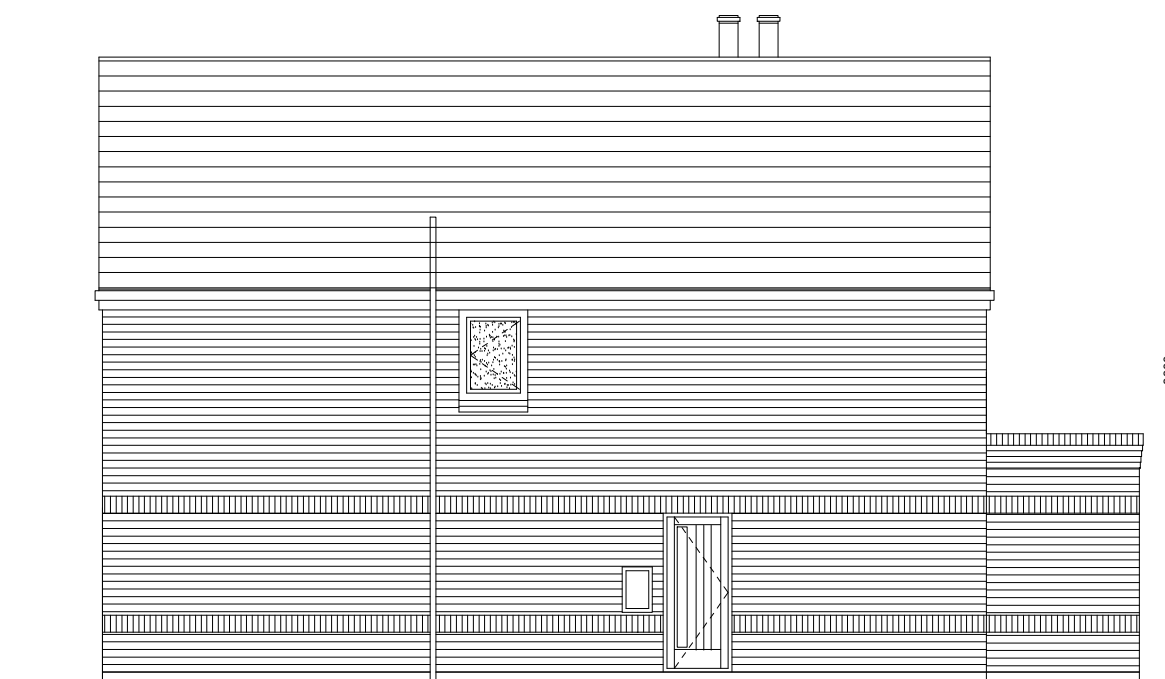
SIDE ELEVATION 2
