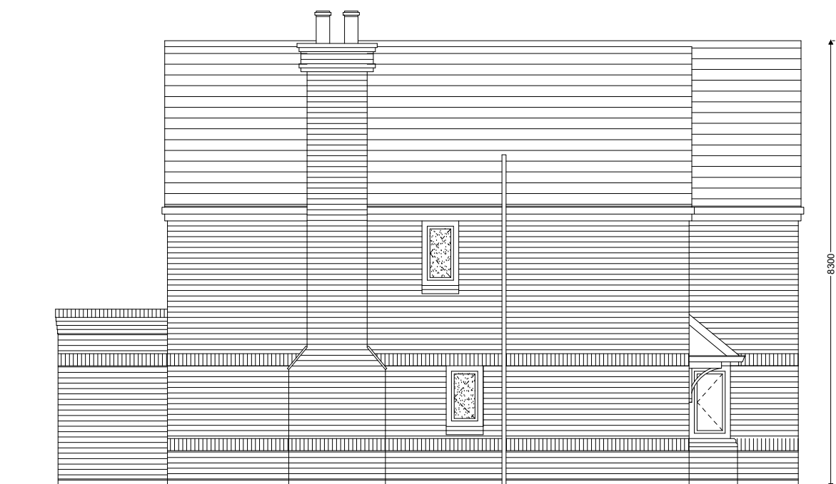
SIDE ELEVATION 1
