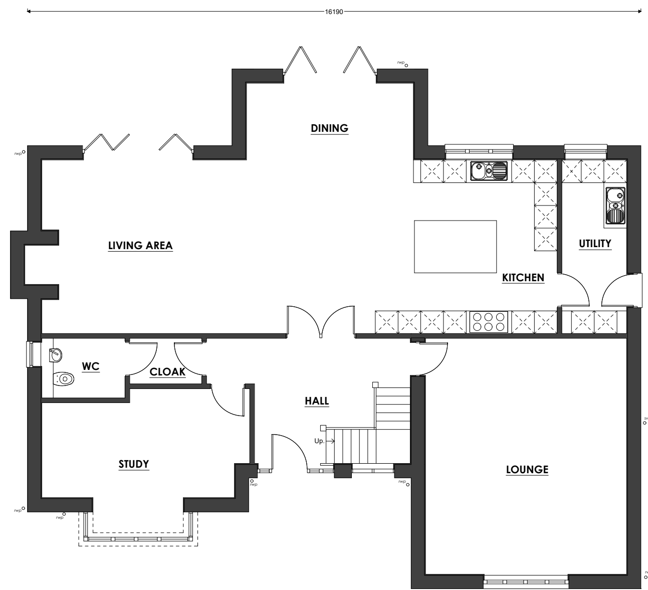
PROPOSED GF PLAN
