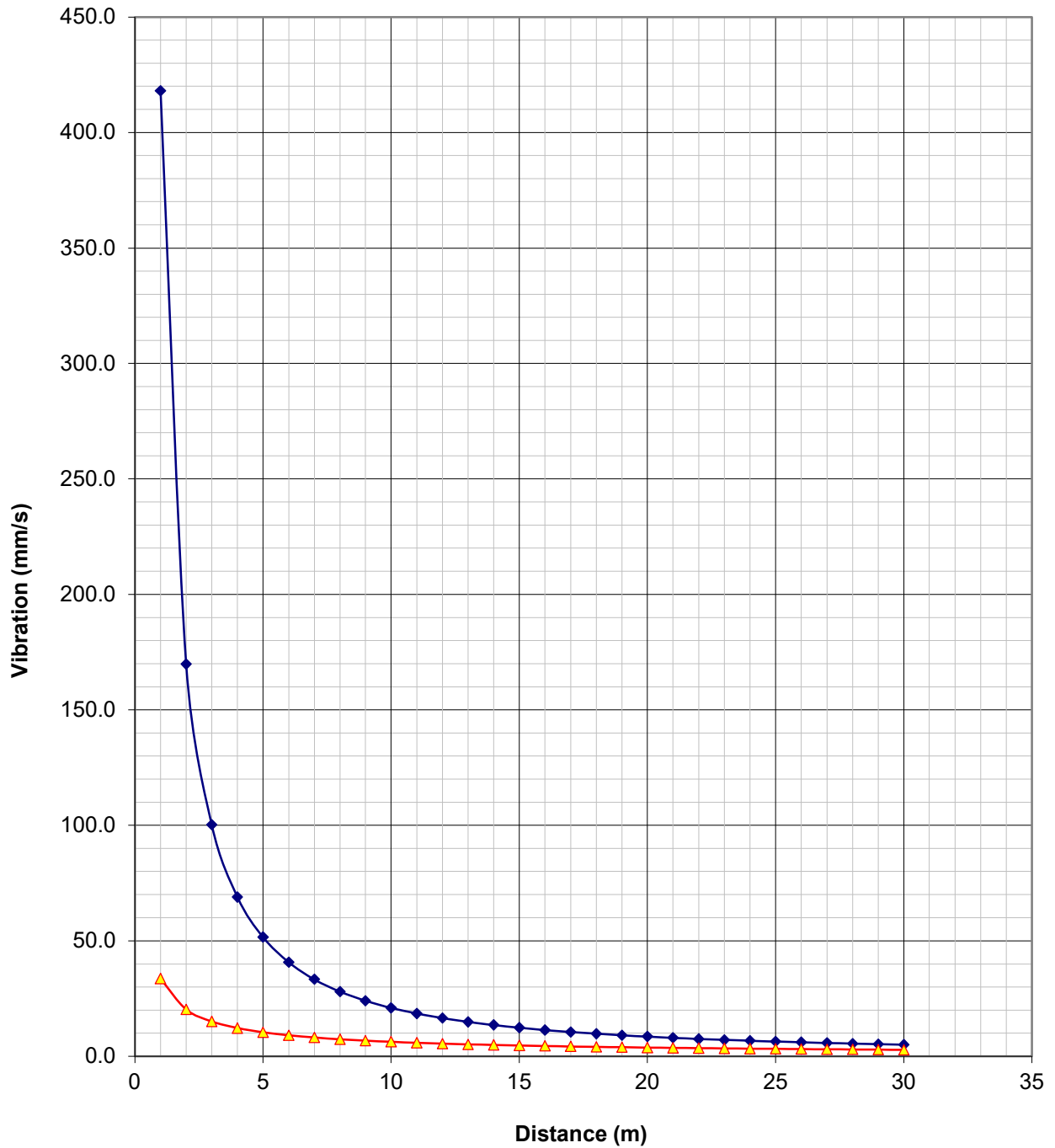
Calculated Vibration Vs. Distance from Source
