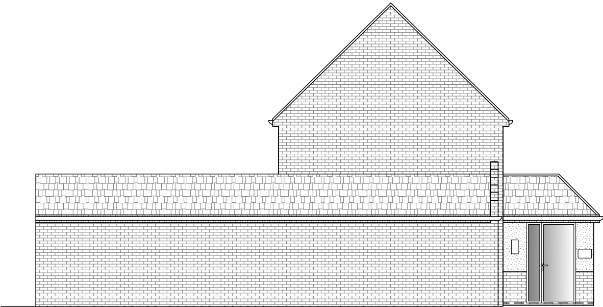
PRE - EXISTING SIDE ELEVATION
