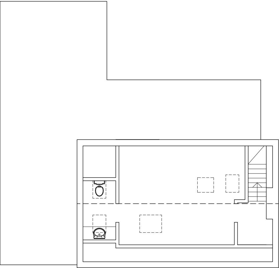
PRE - EXISTING LOFT PLAN
