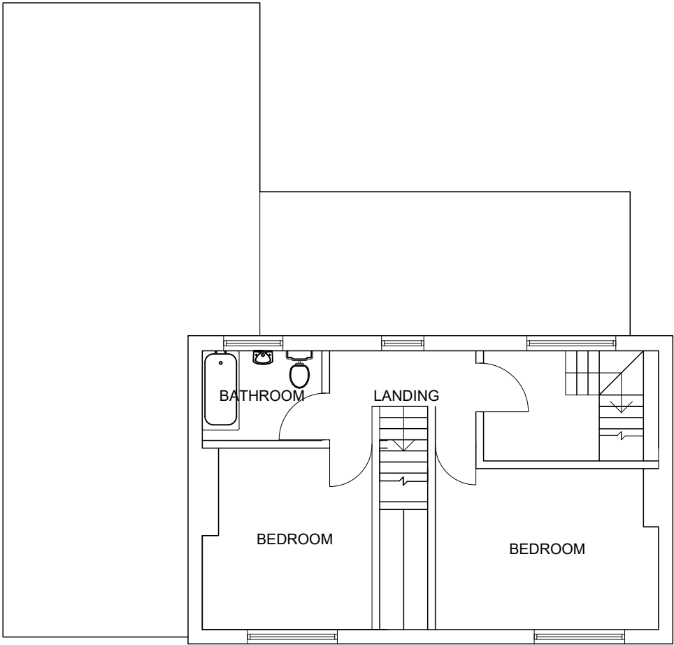
PRE - EXISTING 1st FLOOR PLAN
