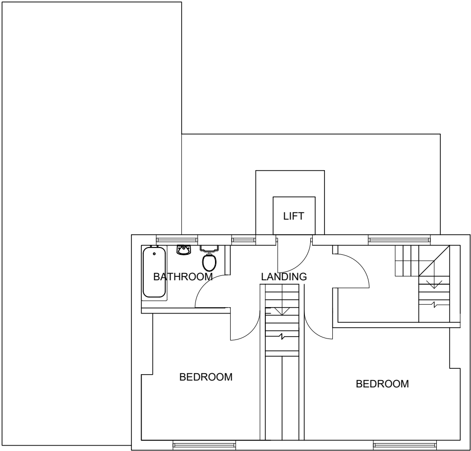
EXISTING 1st FLOOR PLAN
