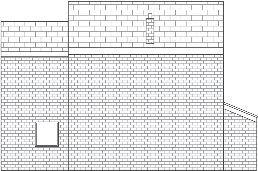
EXISTING SIDE ELEVATION (LEFT TO NO 41)
