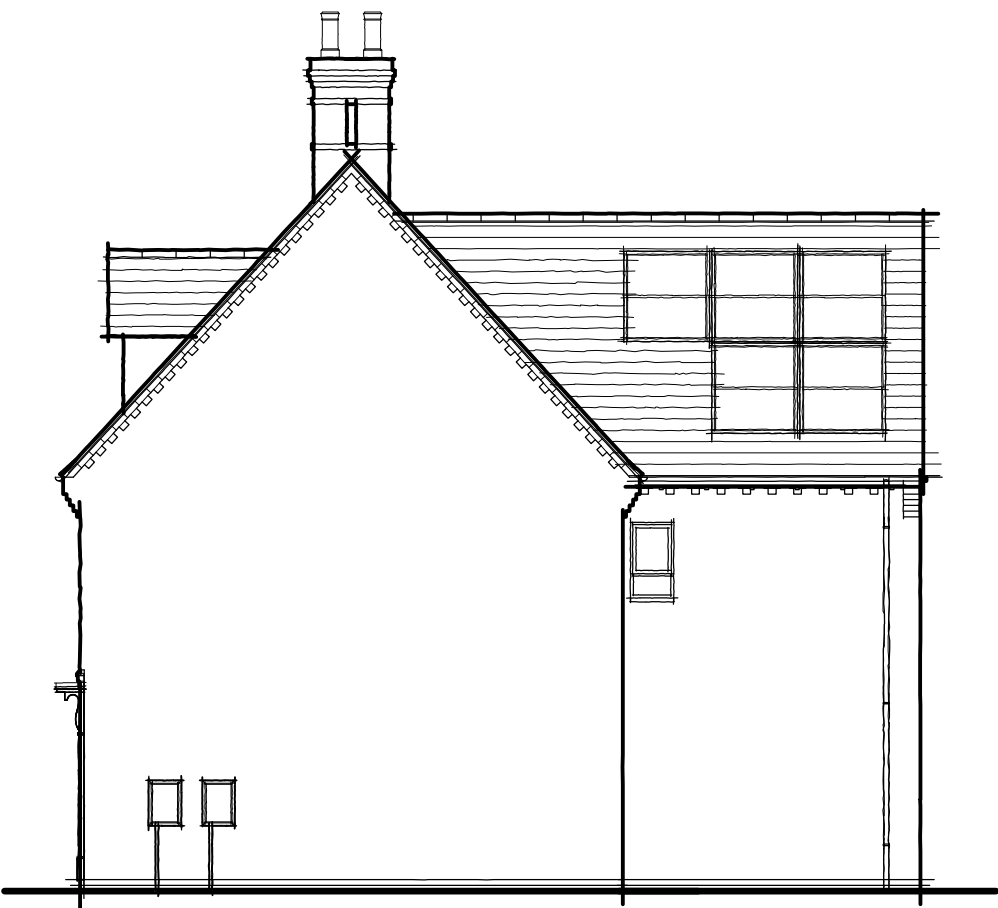
Side Elevation
