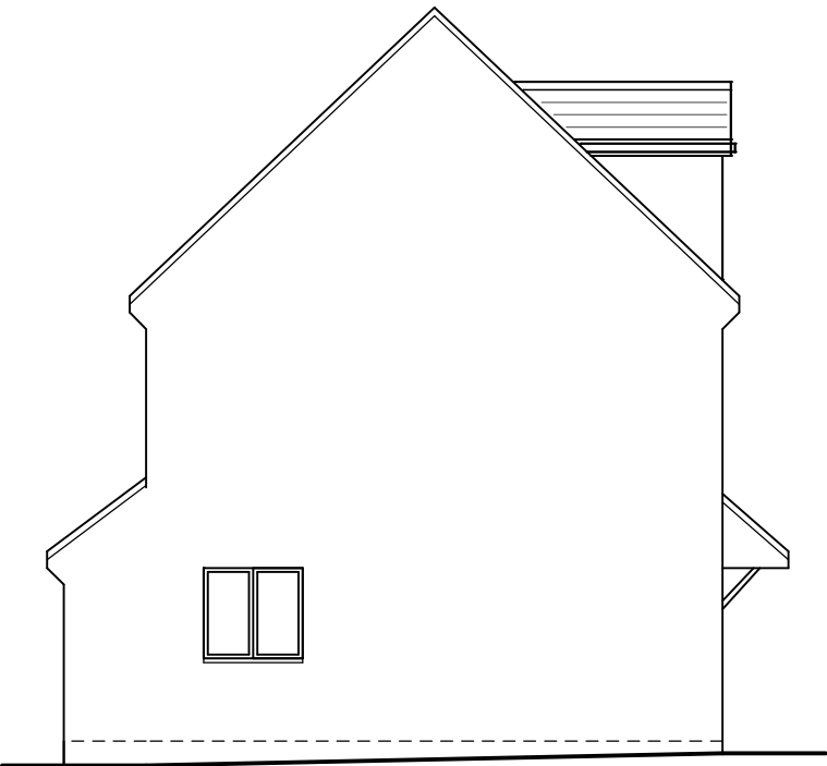
left side (southwest) elevation
