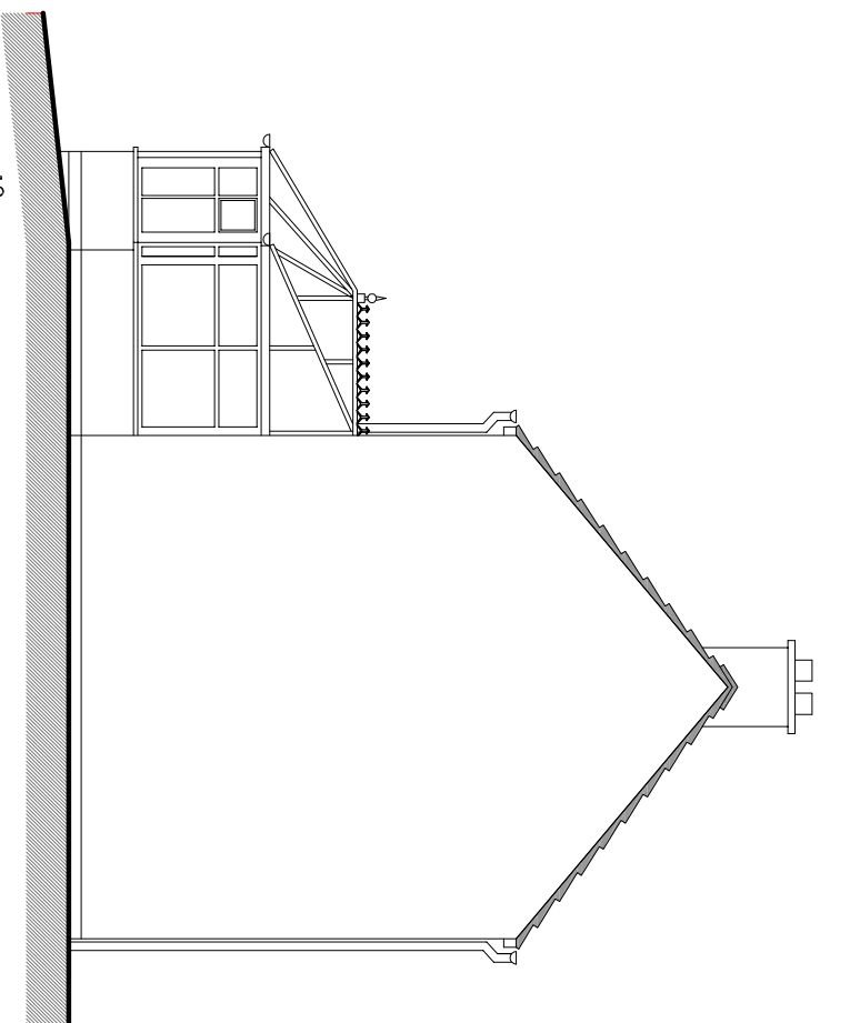
Existing Side Elevation (West Facing)
