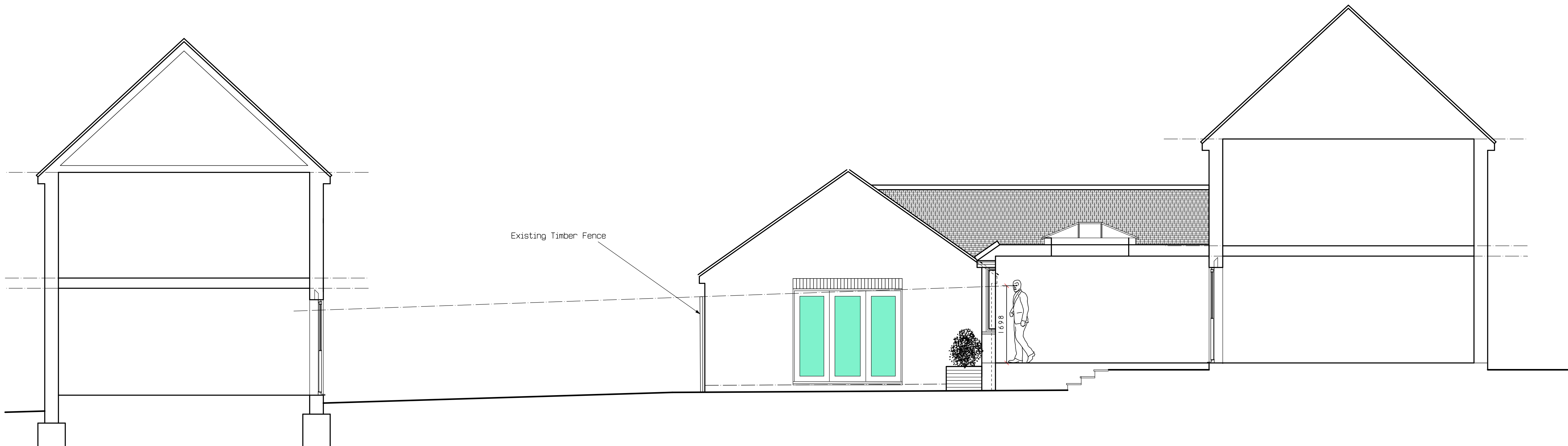
Proposed Section
