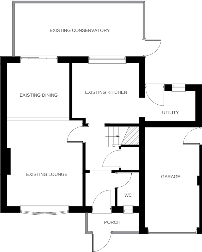
EXISTING GF PLAN 1:100 AT A3
