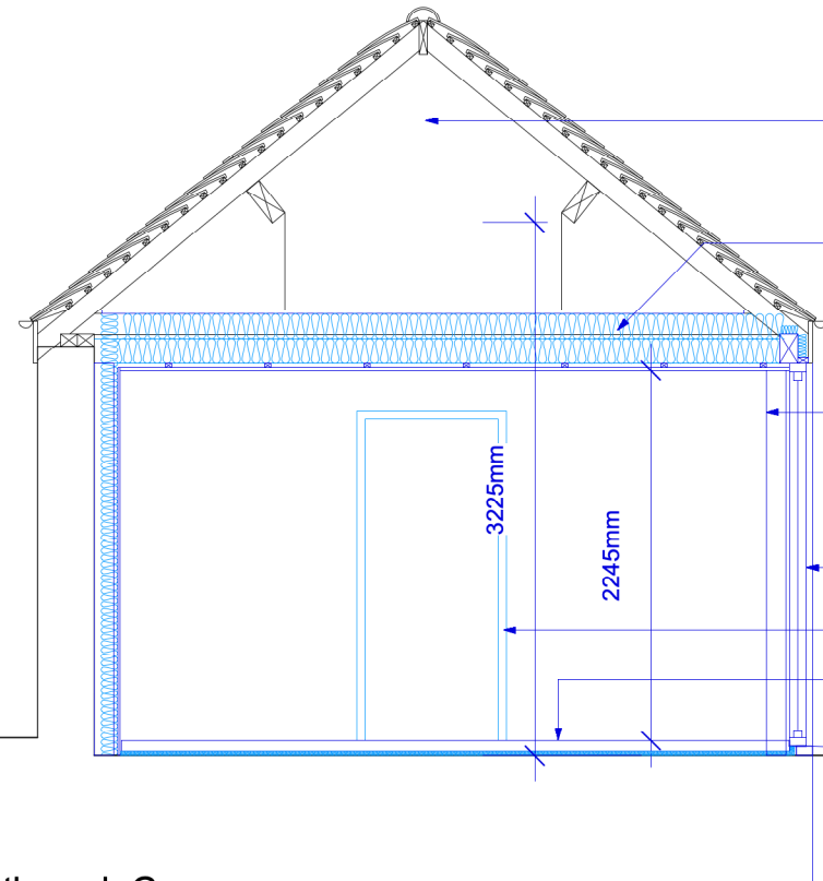
Section through Gym
