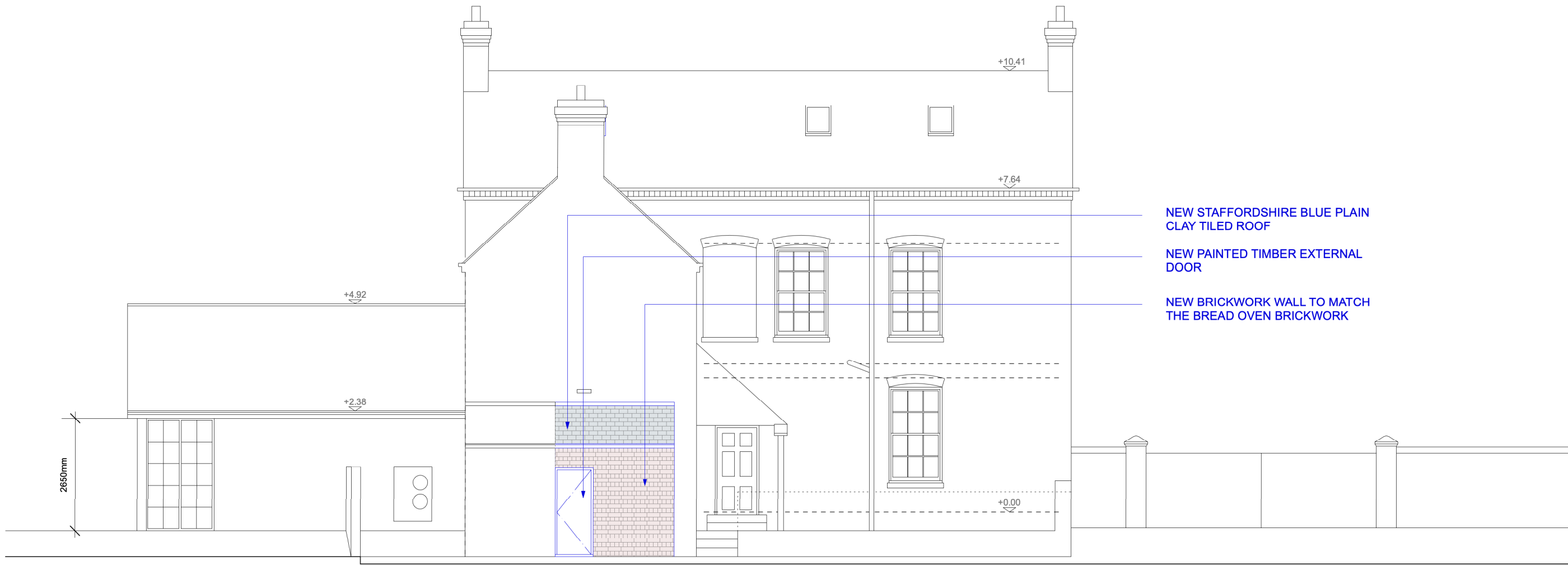
Rear Elevation (facing the garages)
