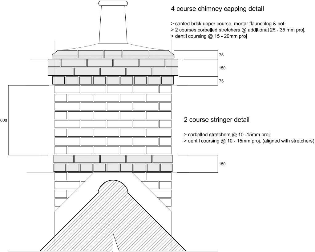
Chimney banding detail 1:20
