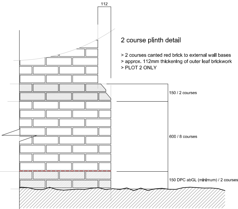
Main wall banding detail 1:20
