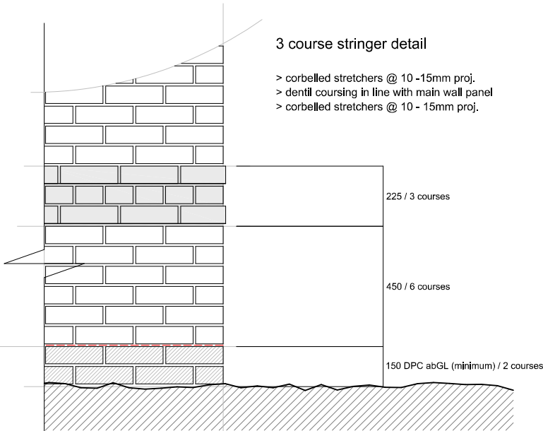
Main wall banding detail 1:20
