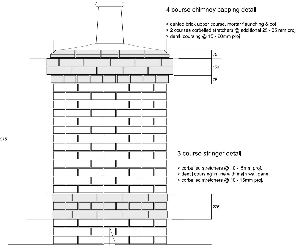
Chimney banding detail 1:20
