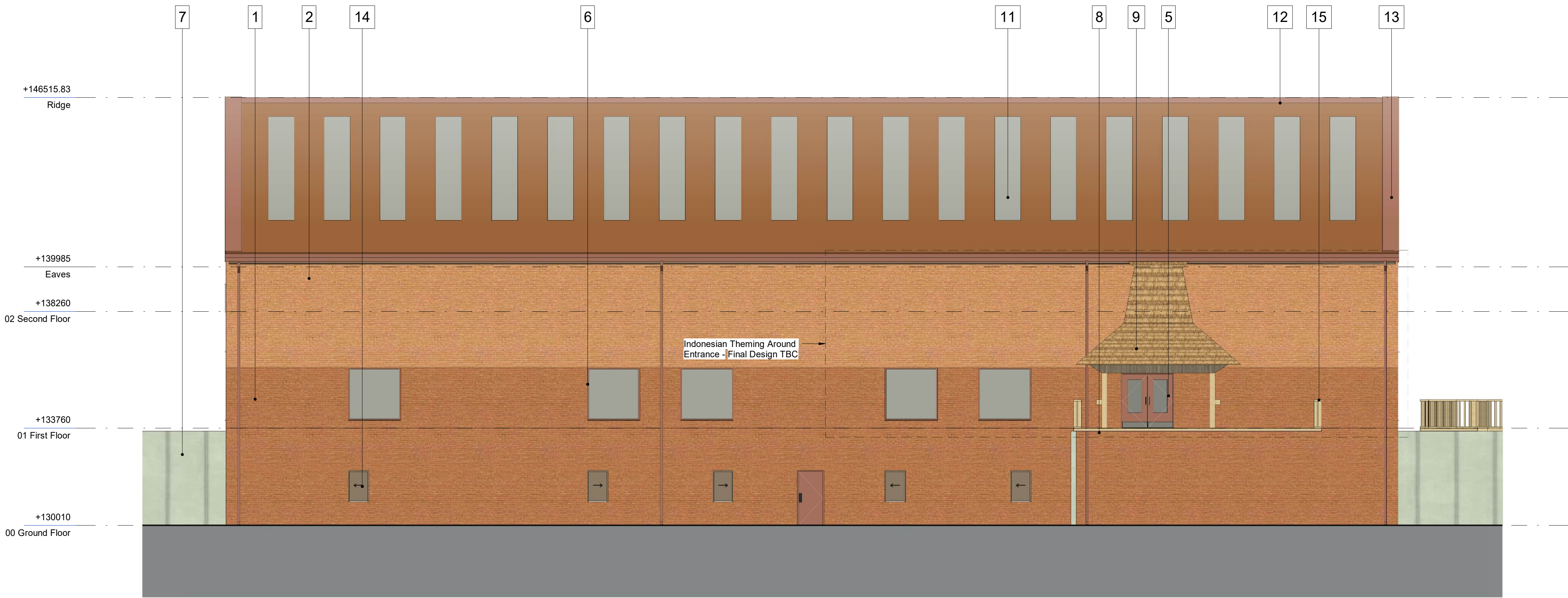
1 Elevation A: South - Orangutan Habitat Building 1 : 100
