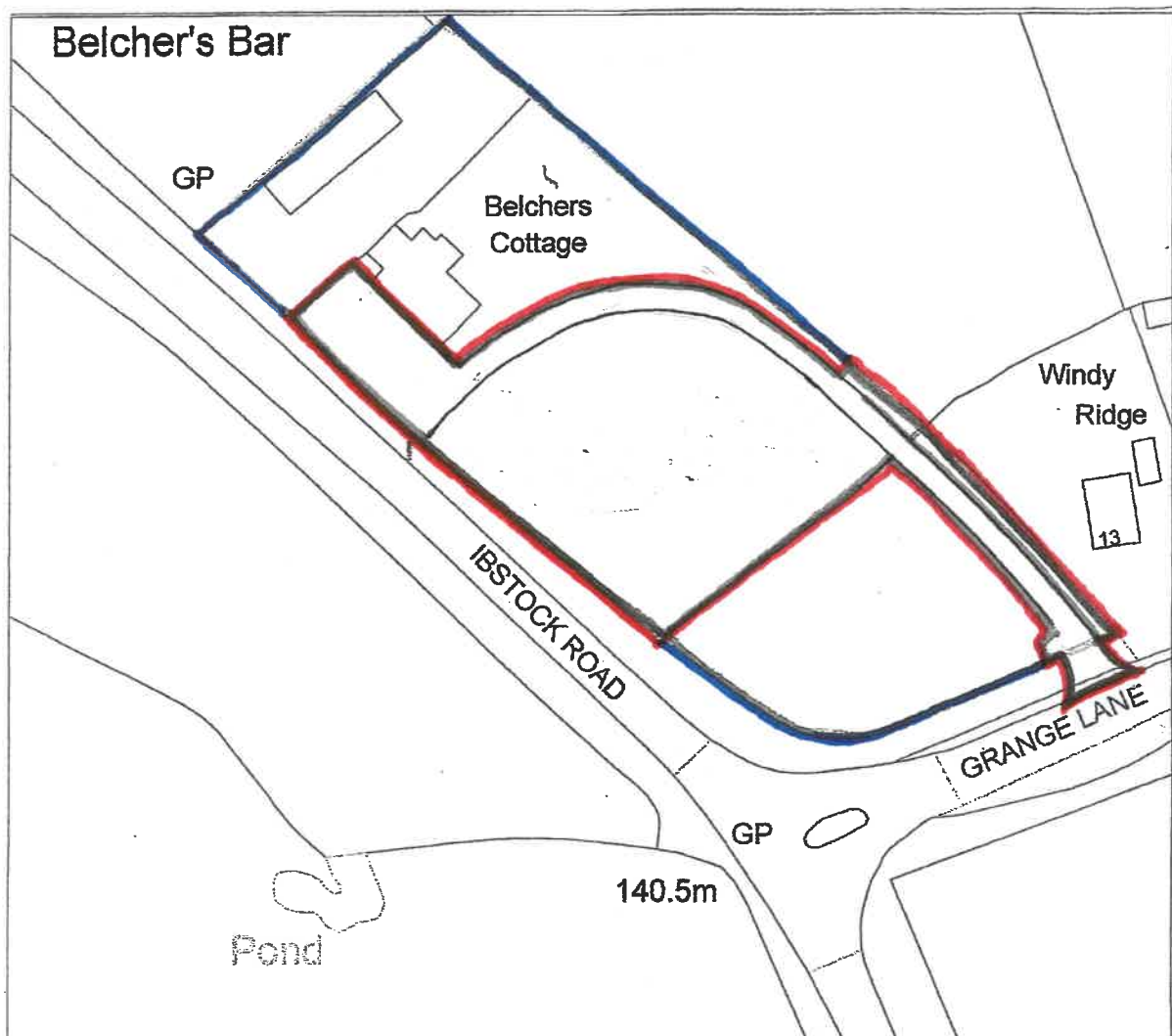
BLOCK/LOCATION PLAN 1:1000
