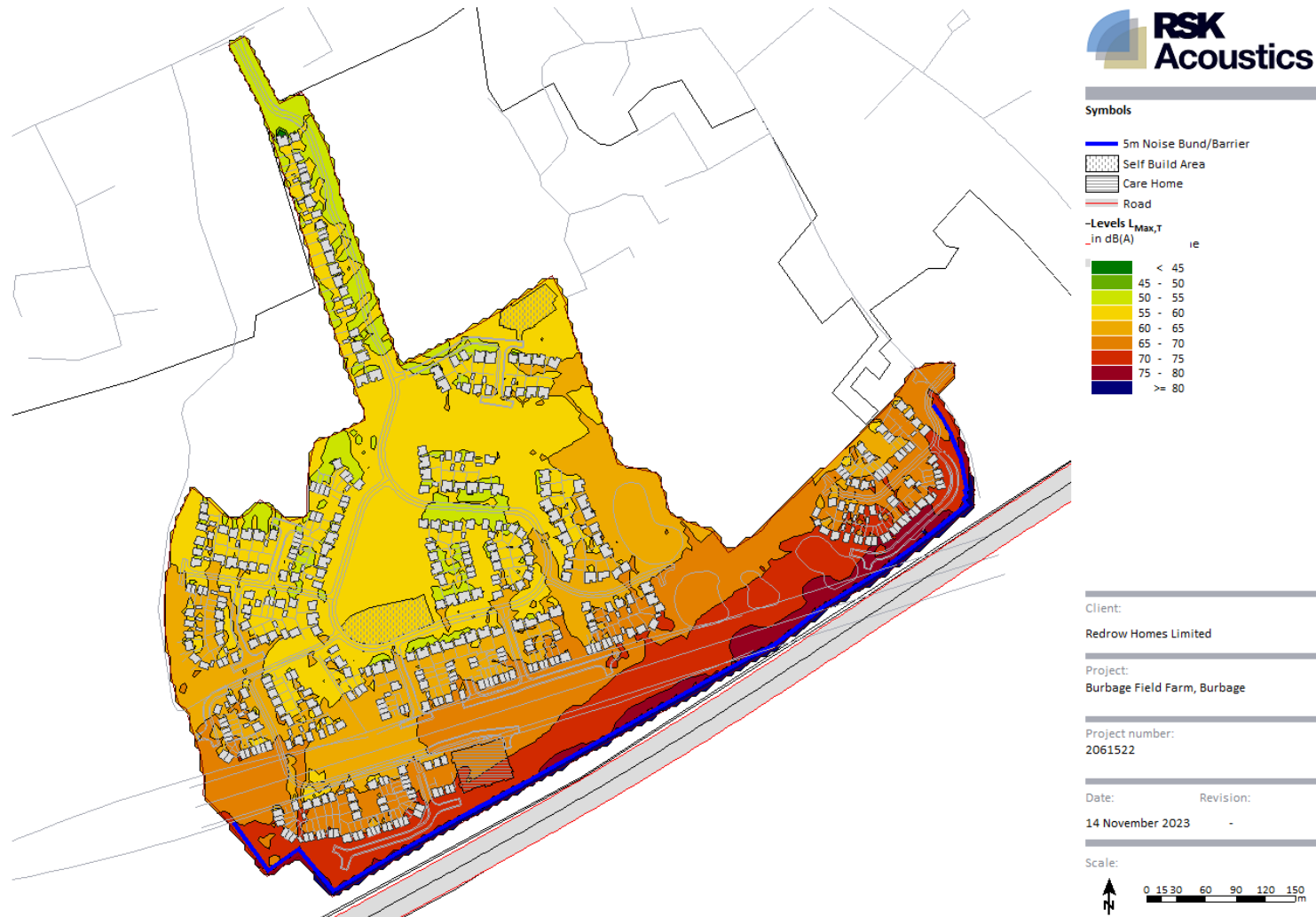
Figure 6 Night-time Maximum Levels, L_{Max}
