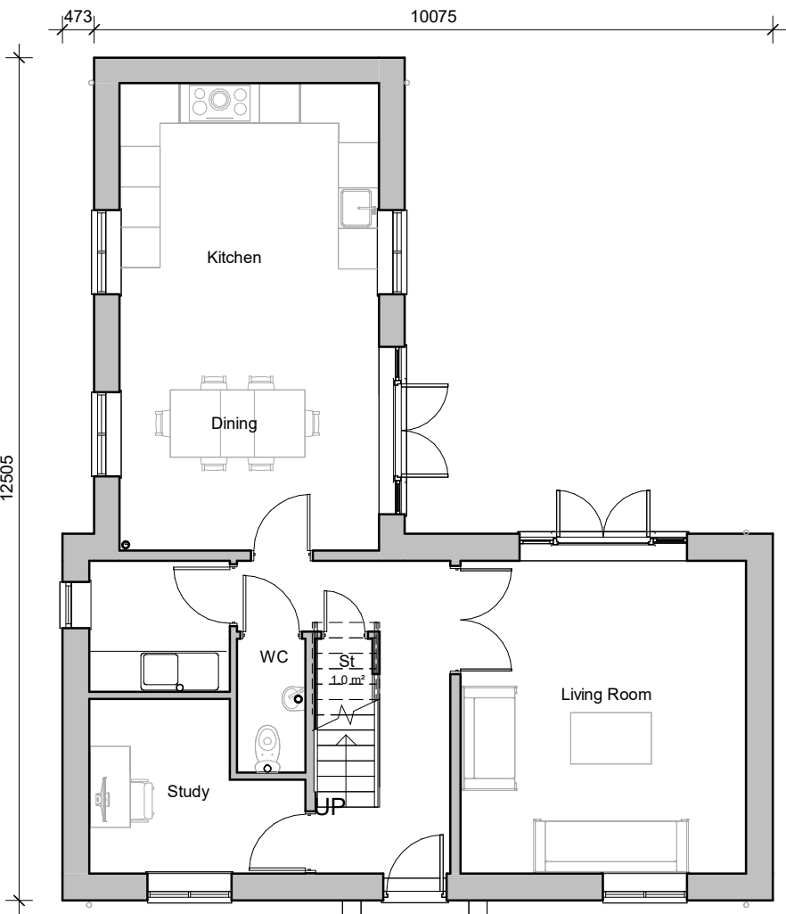
Ground Floor
