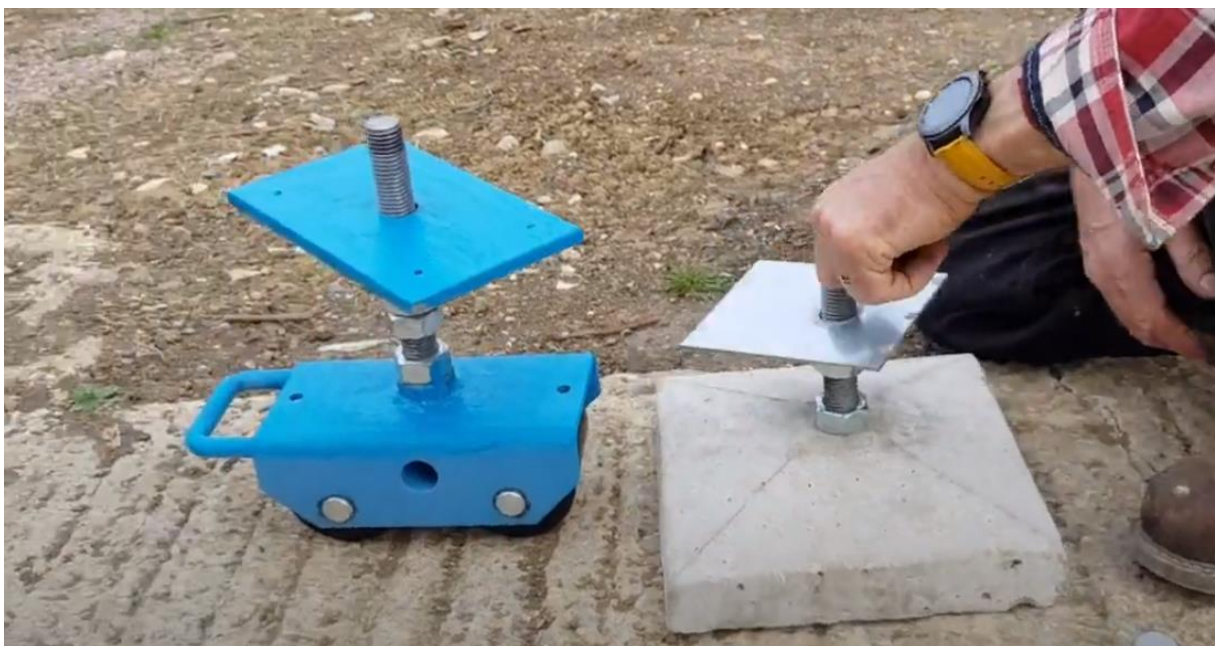
Wheeled foot for moving over ground, and pad foot – each height adjustable to maintain level installation
