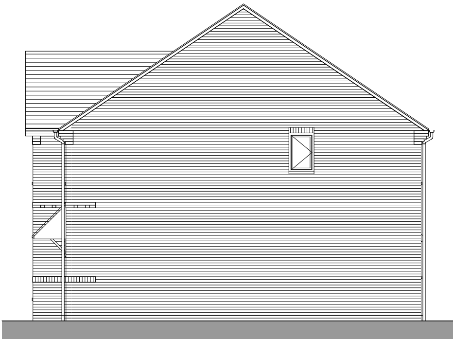
Side Elevation
