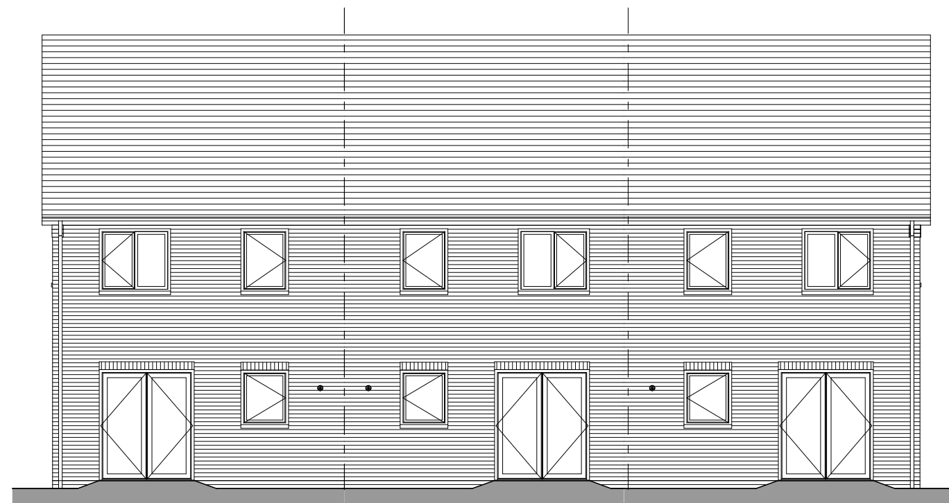
Rear Elevation
