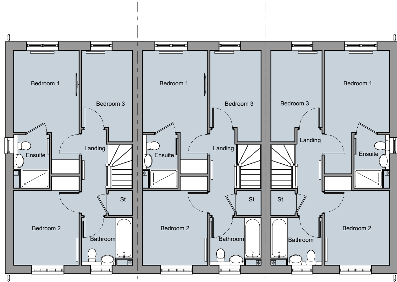
First Floor
