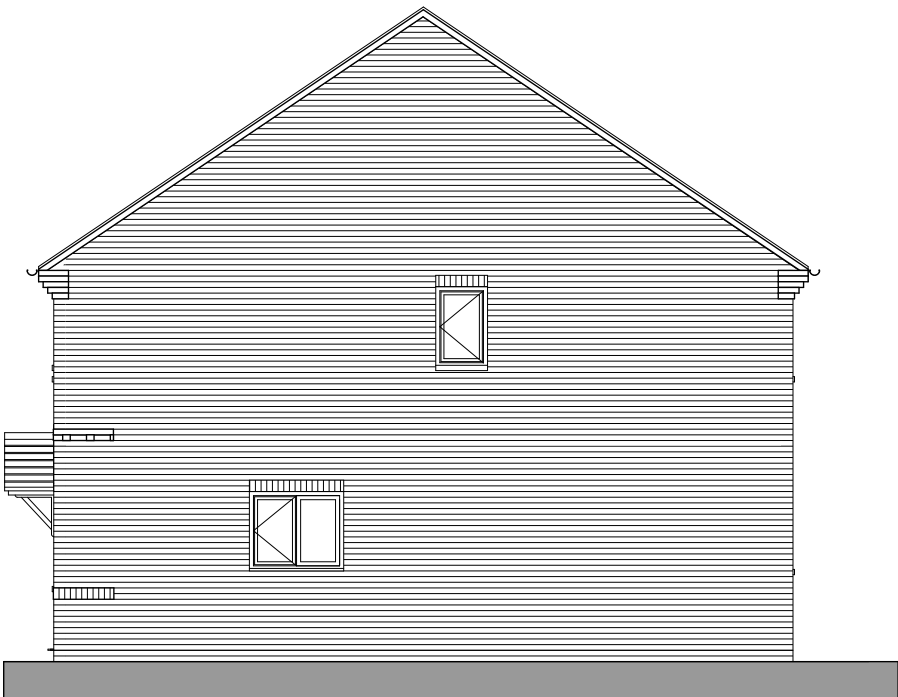
Side Elevation
