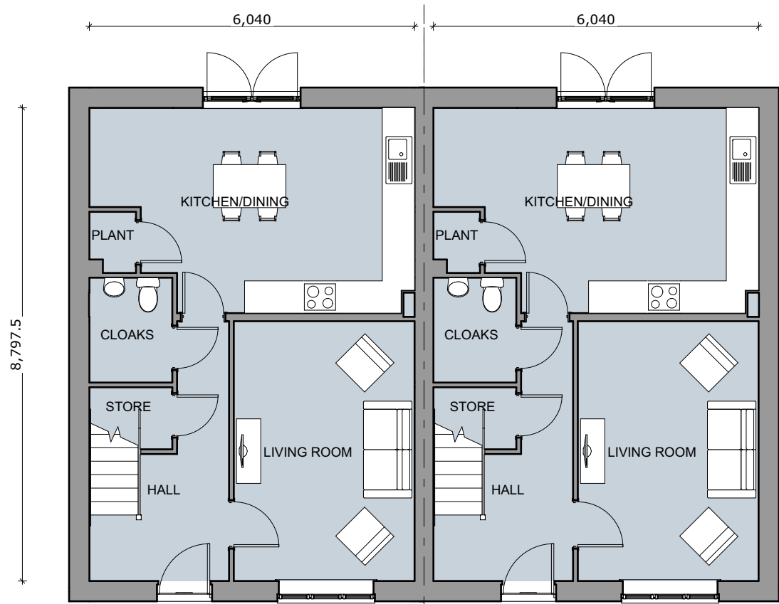
Ground Floor
