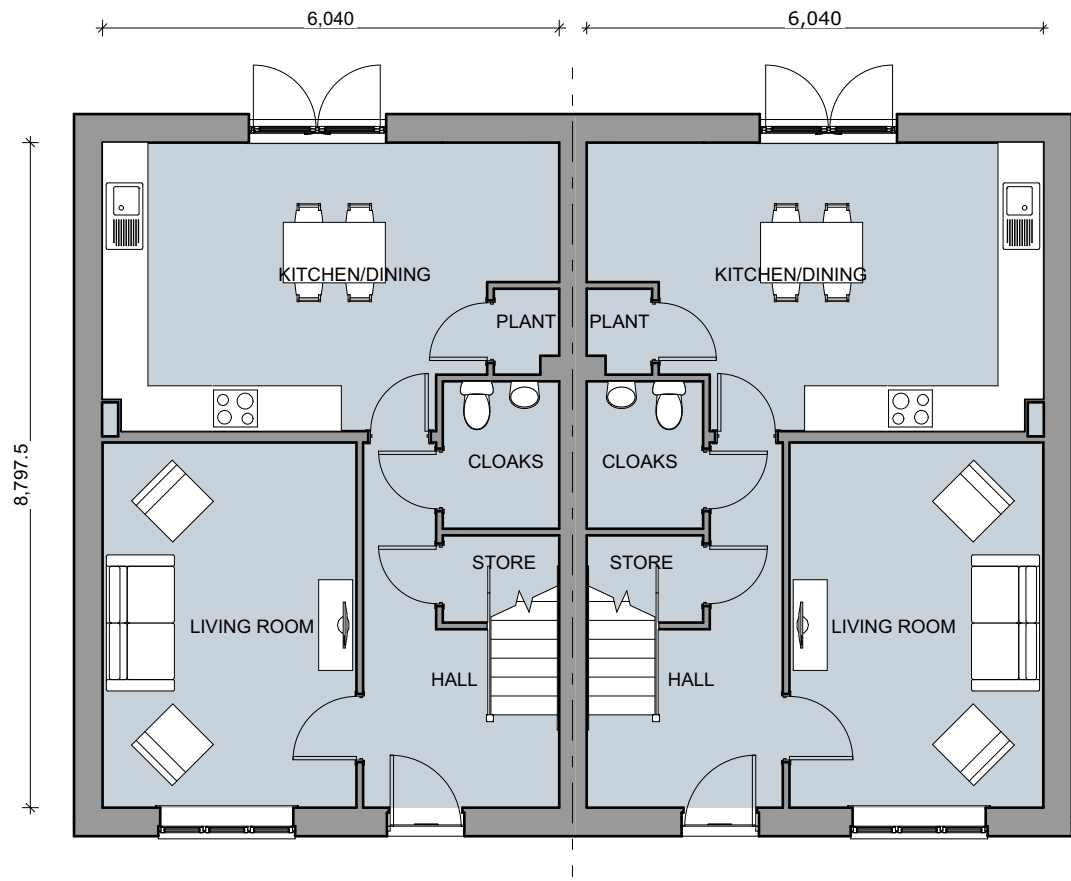
Ground Floor
