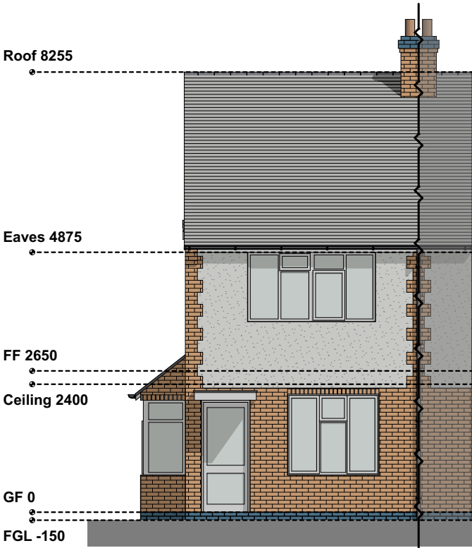
Front Elevation
