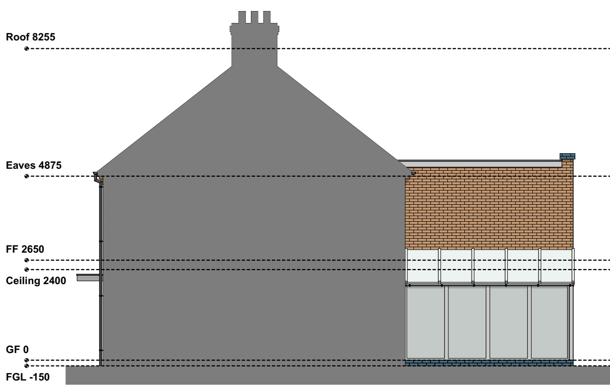
Side Elevation
