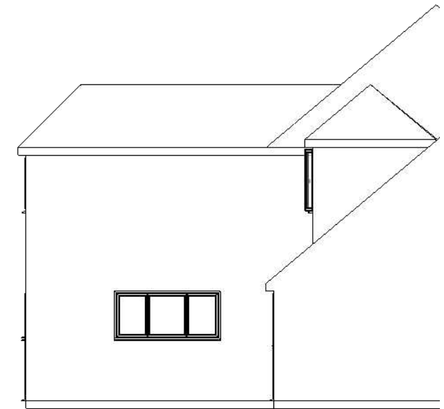
Existing Right Side Elevation
