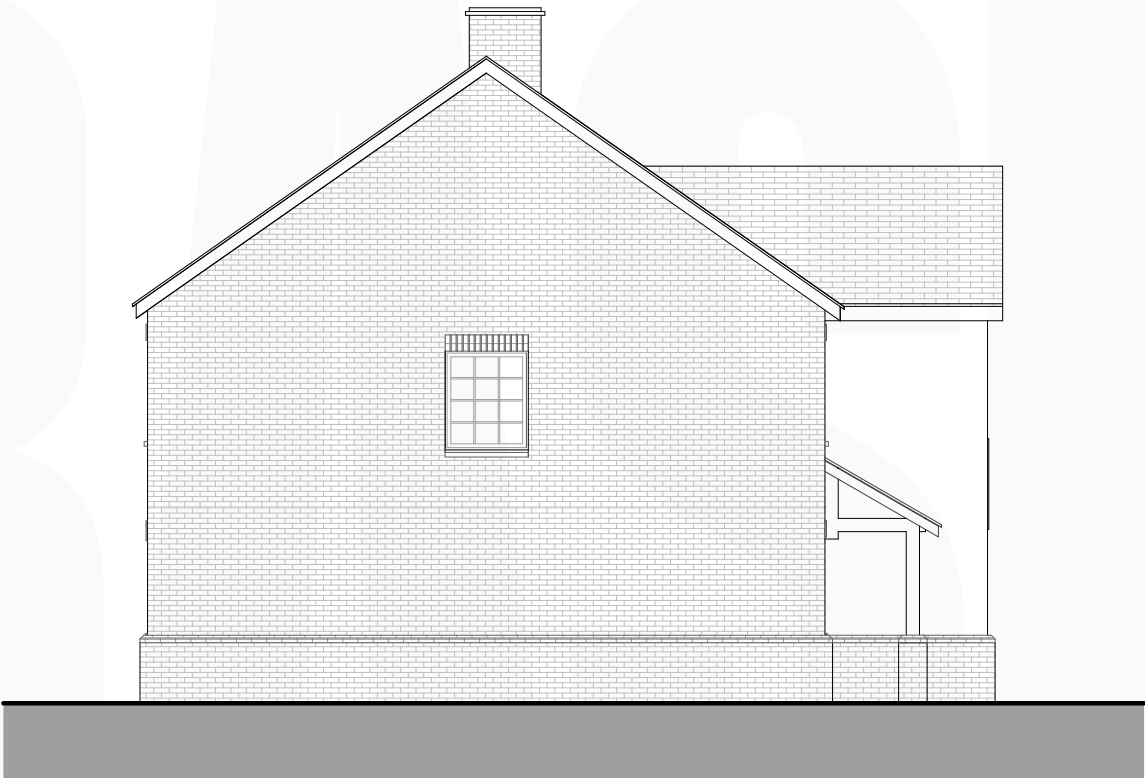
1 Proposed Side Elevation 1:100
