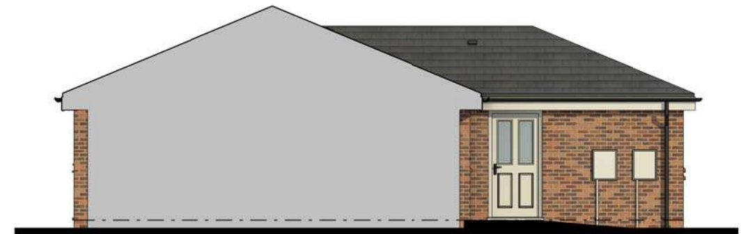
L.H. SIDE ELEVATION - ATTACHED GARAGE
