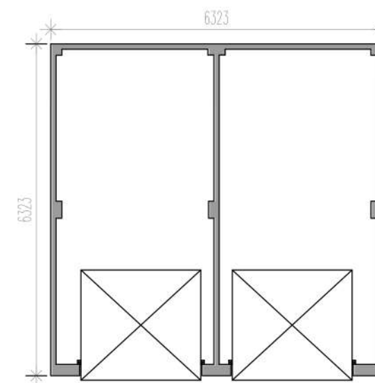
GD30 FLOOR PLAN
