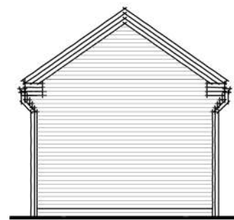
REAR ELEVATION
