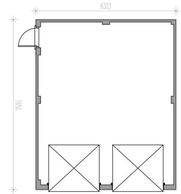
FLOOR PLAN
