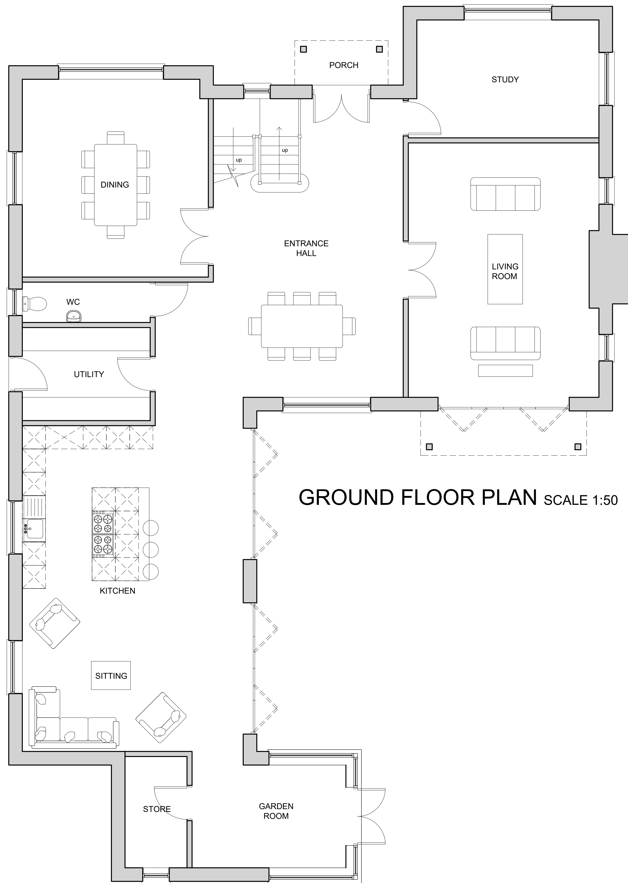
Proposed Floor Plans Scale 1:50
