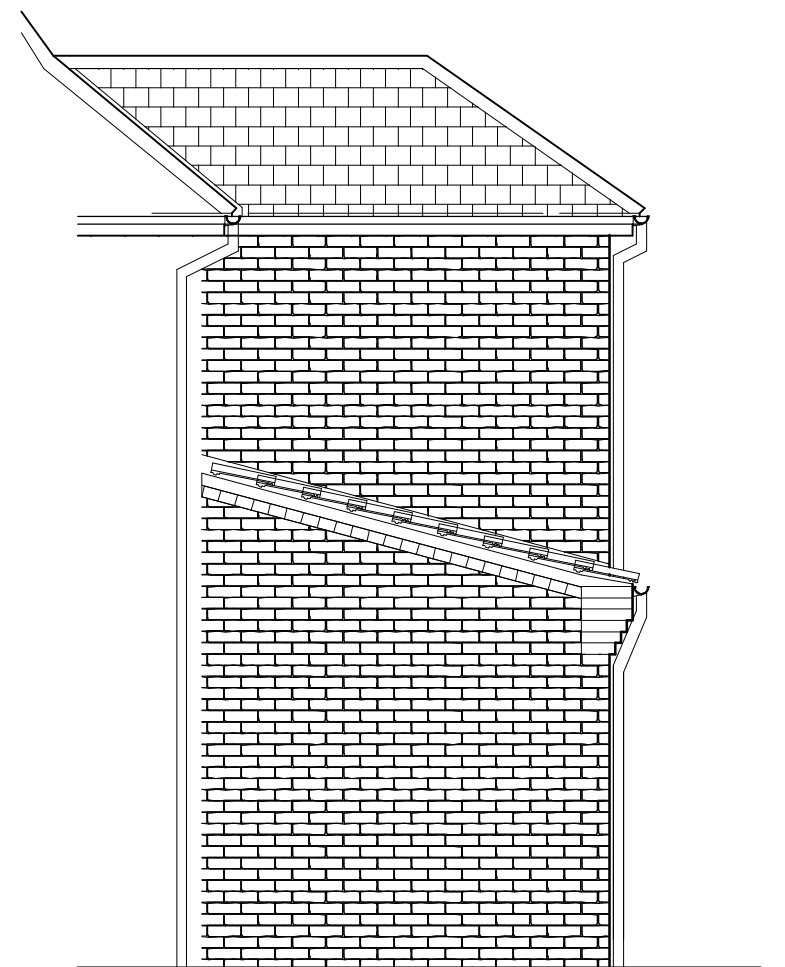
Proposed Side Elevation - north/east
