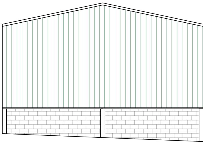
WEST ELEVATION
