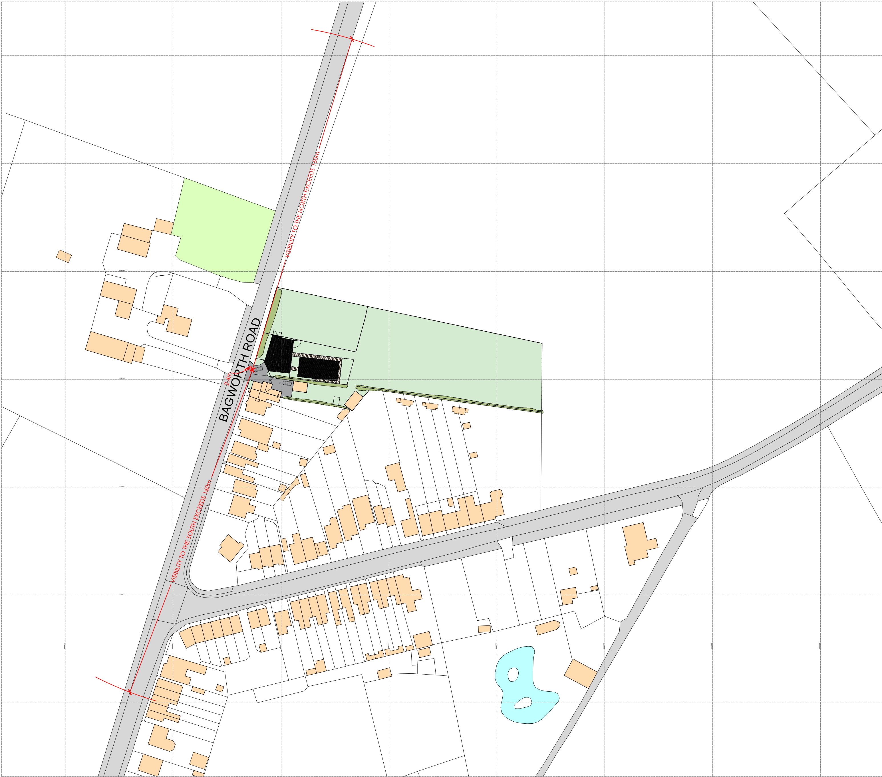
PROPOSED SITE ACCESS/EGRESS VISIBILITY PLAN (1:1000 A1)
