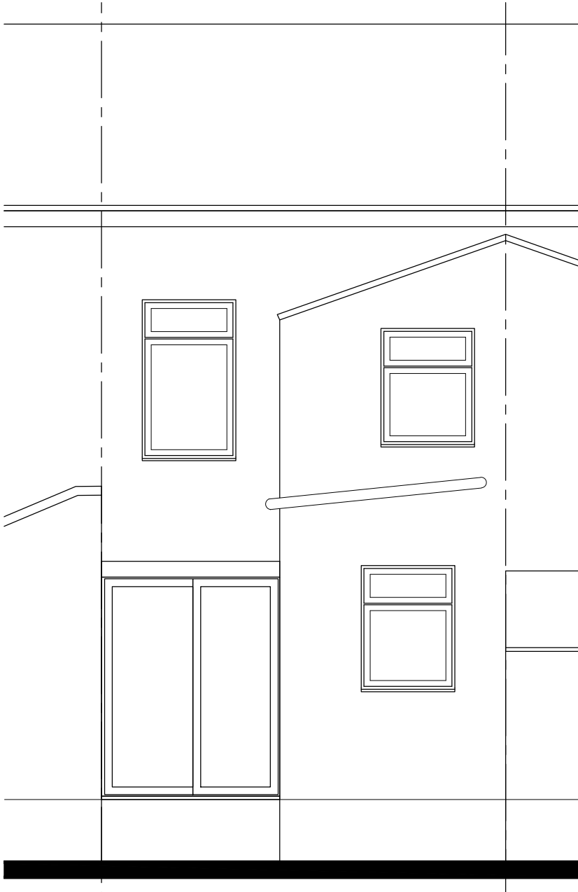
Rear Elevation
