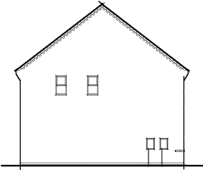
Side Elevation
