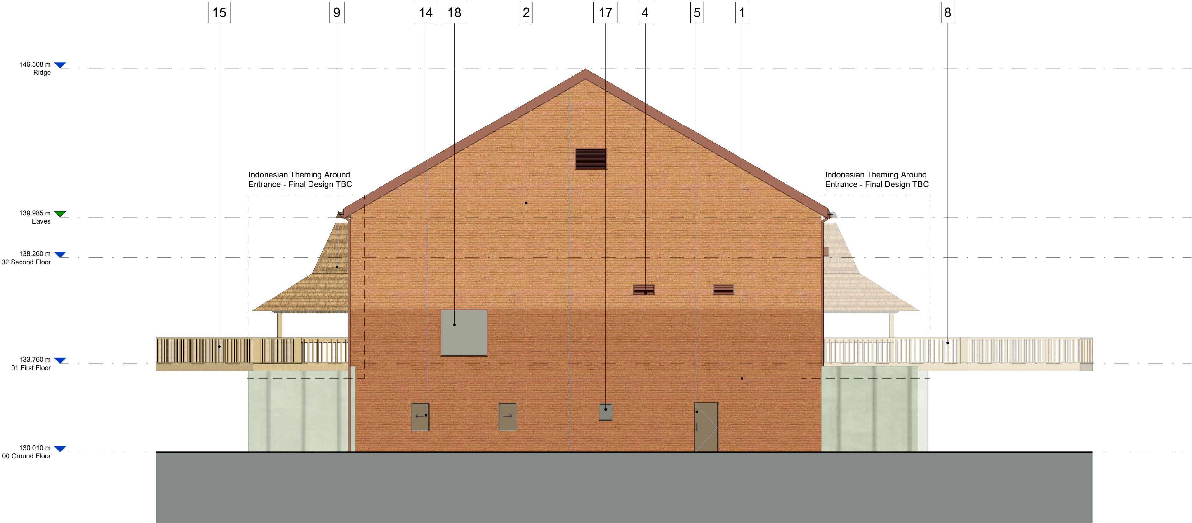
2 00602 Elevation D: East - Orangutan Habitat Building 1 : 100
