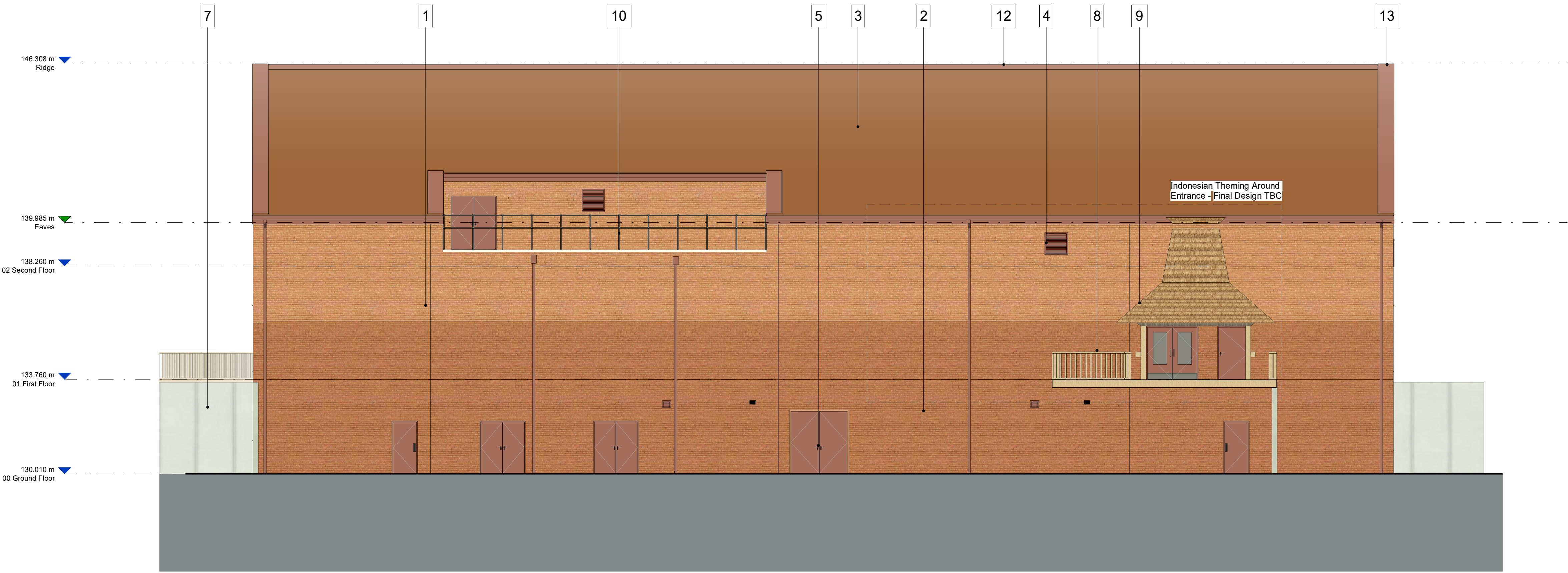
1 00602 Elevation C: North - Orangutan Habitat Building 1 : 100
