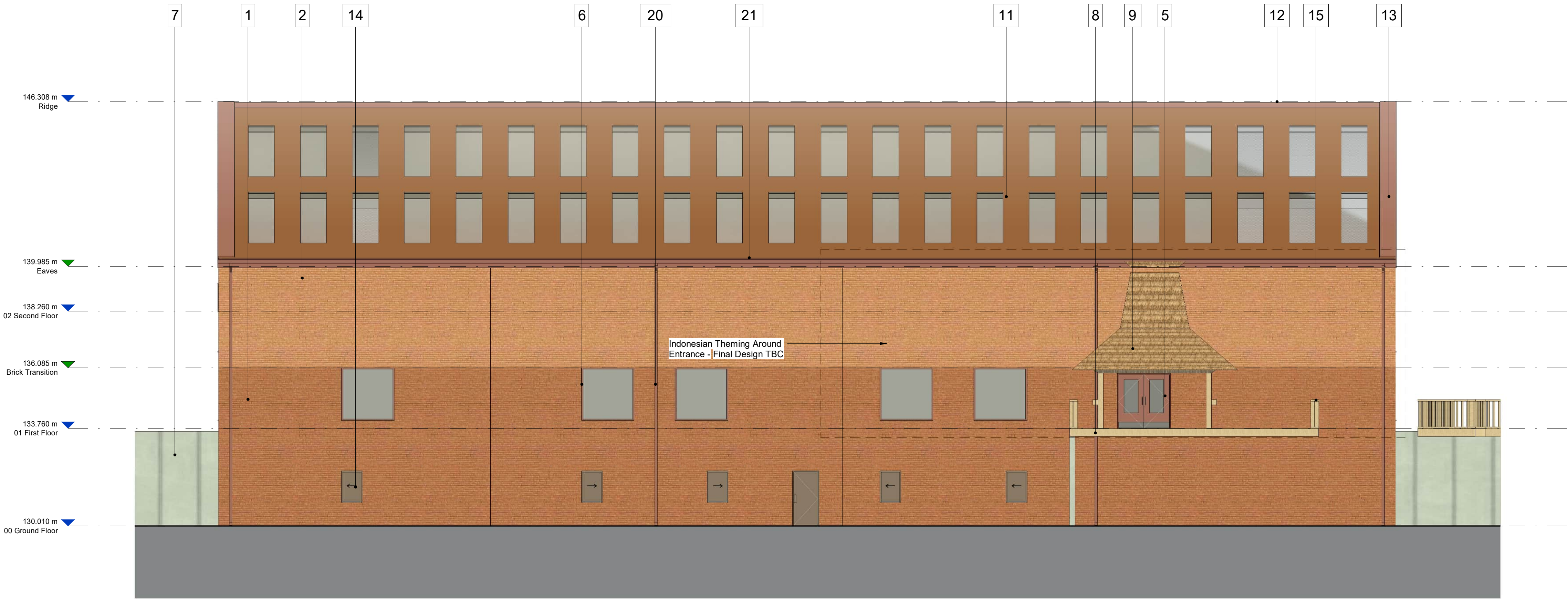
1 Elevation A: South - Orangutan Habitat Building 00601 1 : 100
