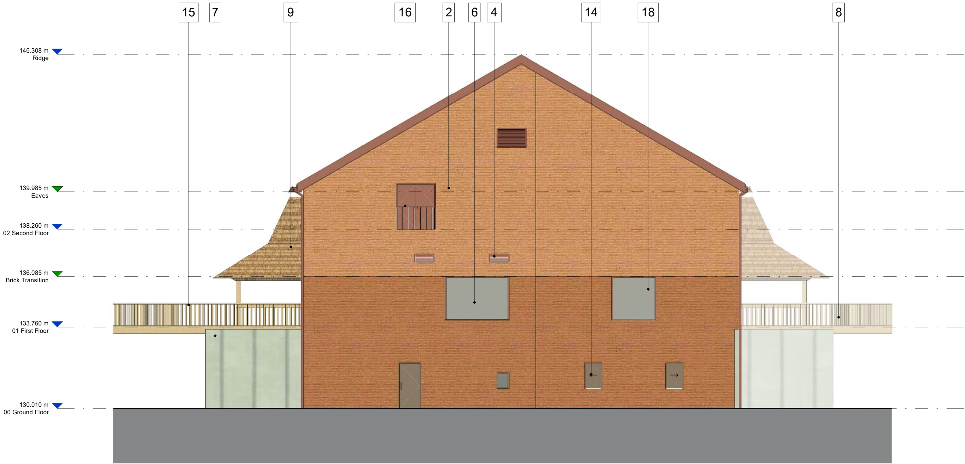
2 Elevation B: West - Orangutan Habitat Building 00601 1 : 100
