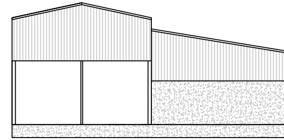
NORTH-WEST ELEVATION
