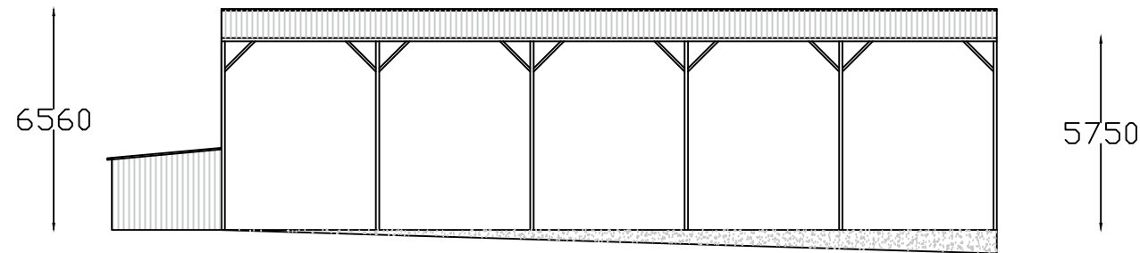
SOUTH-WEST ELEVATION
