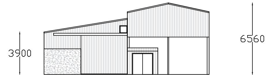
NORTH-WEST ELEVATION
