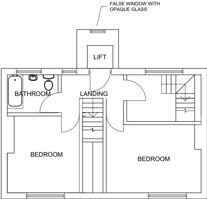
PROPOSED 1st FLOOR PLAN
