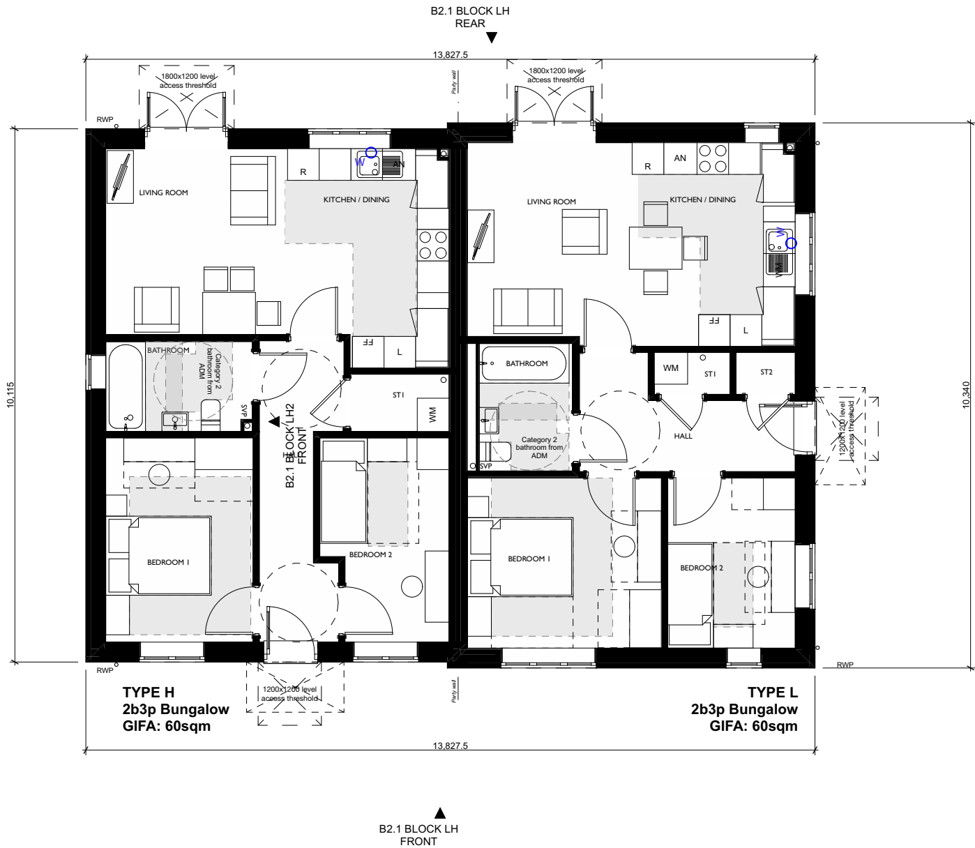
B2.1 BLOCK LH GROUND FLOOR 1:100
