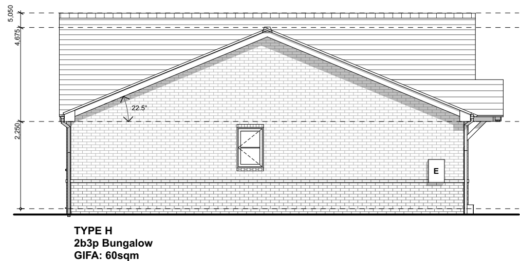
GABLE 1 ELEVATION 1:100
