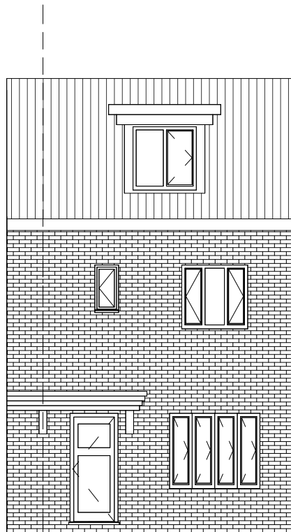
2 Proposed Front Elevation 1 : 100
