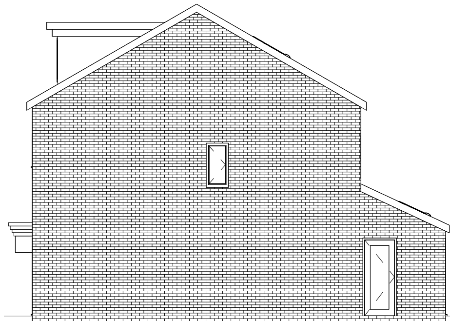
4 Proposed Side A Elevation 1 : 100
