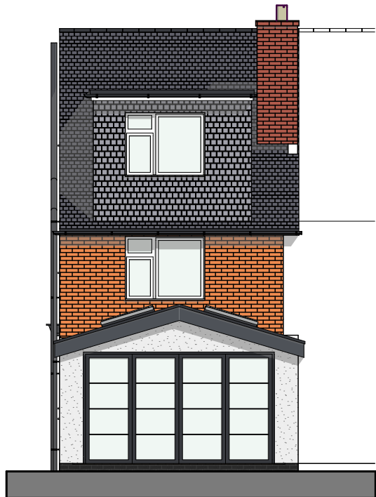
Rear Elevation
