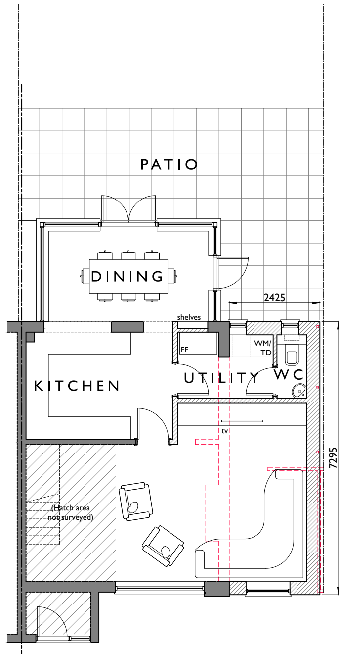
Proposed - Ground Floor Plan 1:100 0 1m 2m 3m 4m 5m NORTH
