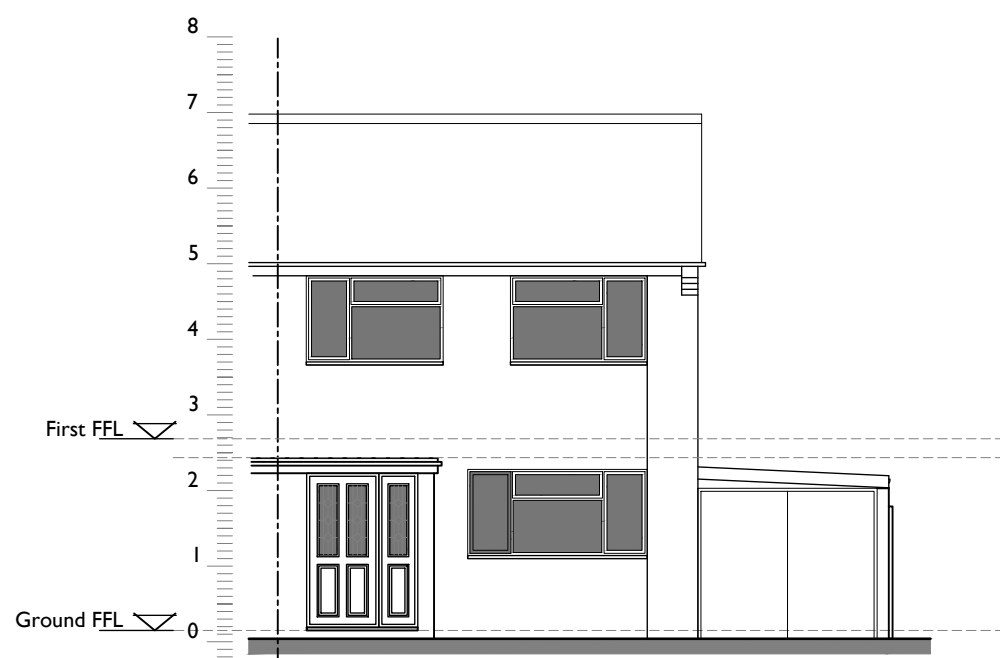
Existing - North Elevation 1:100
