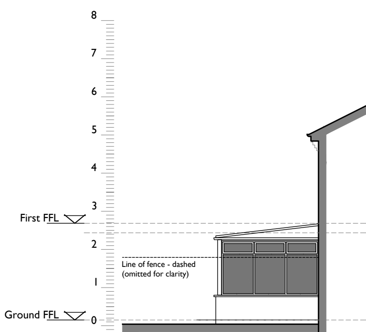
Proposed - East Elevation 1:100
