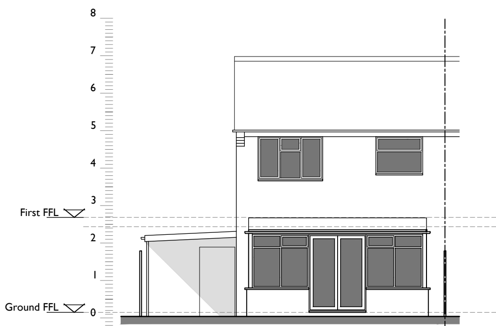
Existing - South Elevation 1:100
