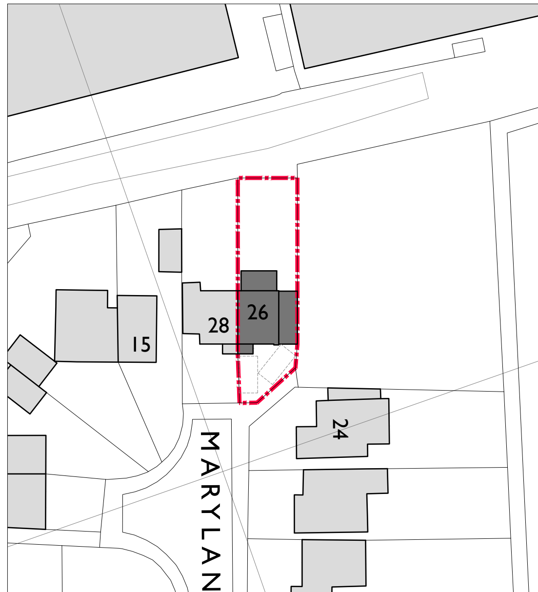
Site Plan 1:500 0 5m 10m 15m 20m 25m 30m NORTH
