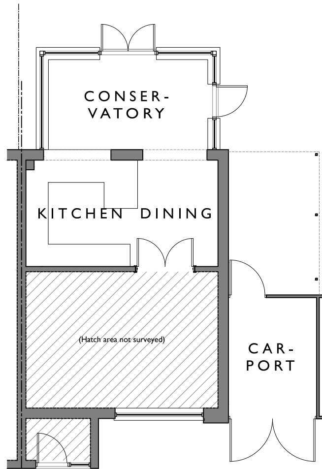
Existing - Ground Floor Plan 1:100 0 1m 2m 3m 4m 5m NORTH
