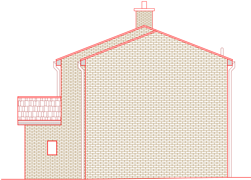
PROPOSED SIDE ELEVATION-1
