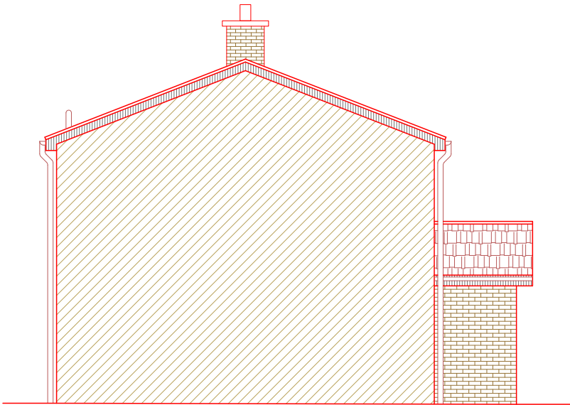
PROPOSED SIDE ELEVATION-2
